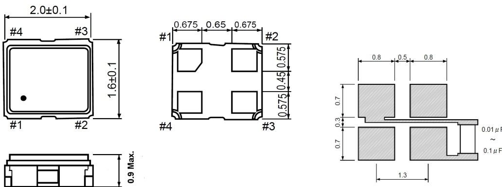
Figure 2) Suggested Land Pattern
