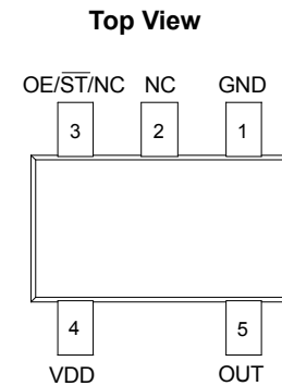
Figure 1. Pin Assignments
