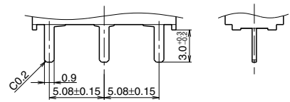
PC board terminal
