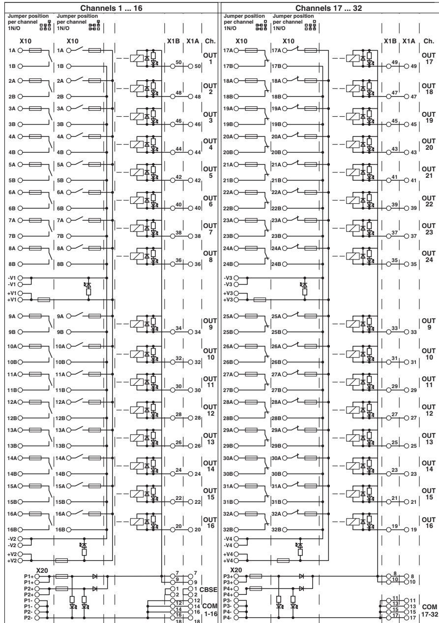
Circuit diagram
