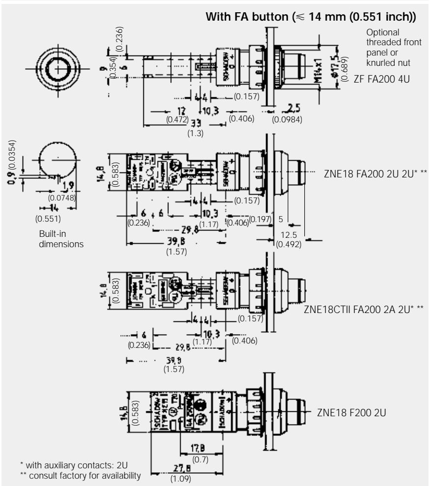
Push-button switches with central mounting: ZF, ZNE18 and ZNE18CTII with F200 or FA200 button (14 mm (0.551) diameter)
