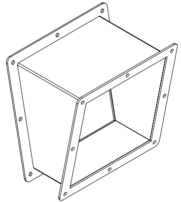
ISOMETRIC VIEW
