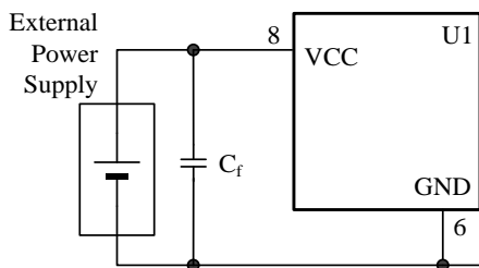
Figure 9-3 The VCC pin peripheral circuit
