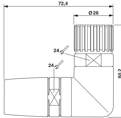
Dimensioned drawing
