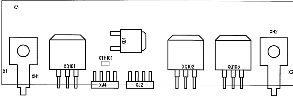
Primary IMS board
