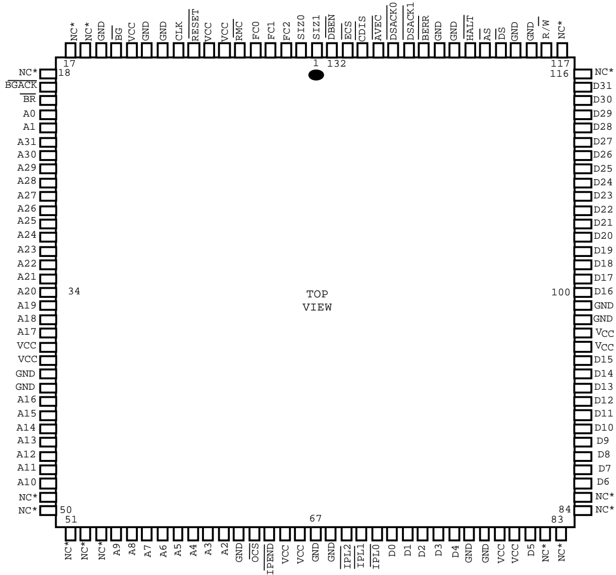
Figure 1. FC and FE Suffix Pin Assignment
