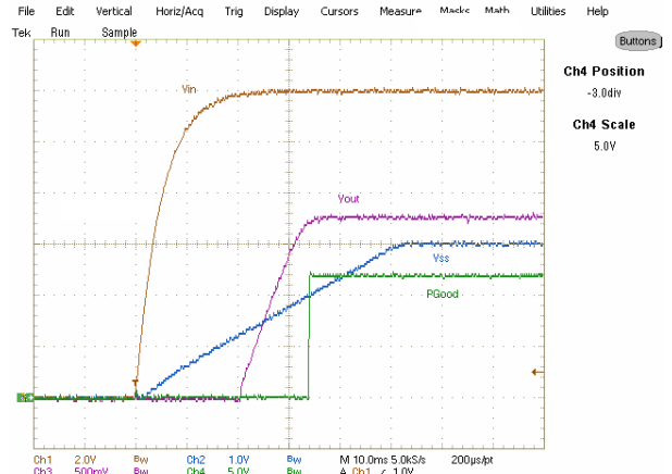
Fig. 8: Start up at 4A Load, Ch 1 :V in , Ch 2 :V SS , Ch 3 :V out , Ch 4 :V PGGood
