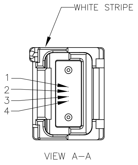
LIGHTRAY MPX CONNECTOR FIBER PATH
