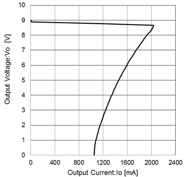
Figure 16. Load Regulation
