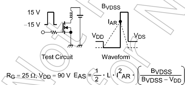
Fig. 8.16 Test Circuit/Waveform
