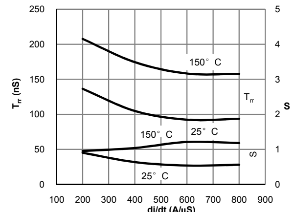
Fig 25: Diode Reverse Recovery Time and Softness Factor vs. di/dt ( V_{GE}=15V, V_{CE}=400V, I_F=30A )
