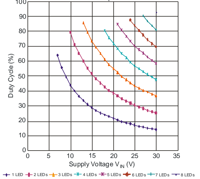
ZXLD1360 Duty Cycle L = 47 \mu H
