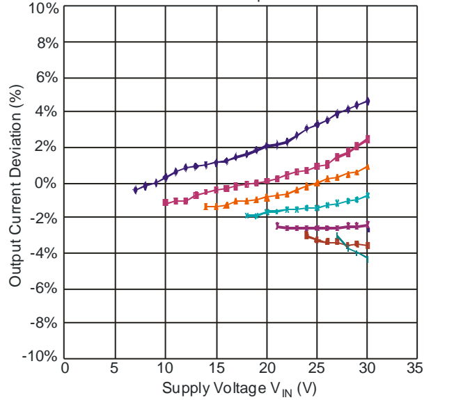
ZXLD1360 Output Current L = 47 \mu H
