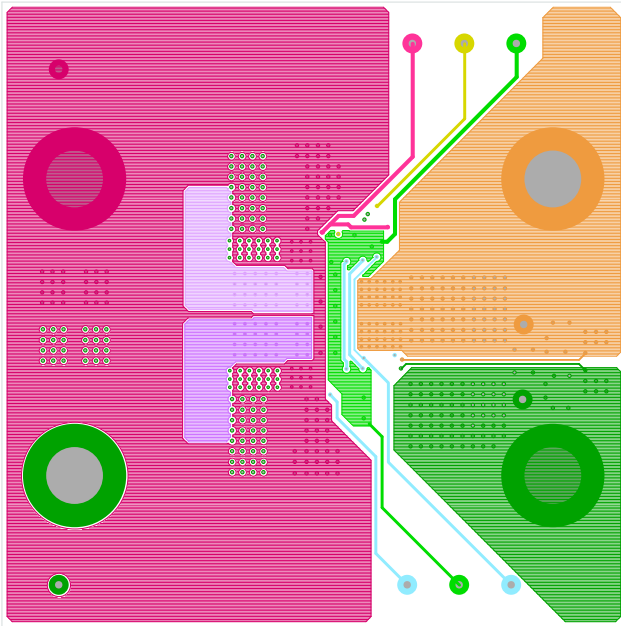
FIGURE 7. LAYER 4
