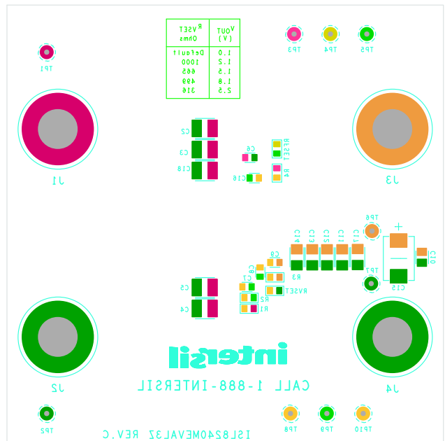
FIGURE 10. SILKSCREEN BOTTOM
