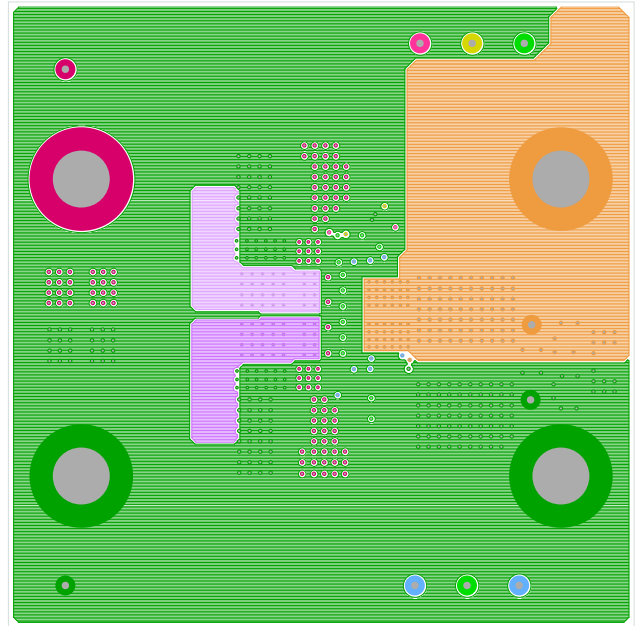
FIGURE 8. LAYER 5
