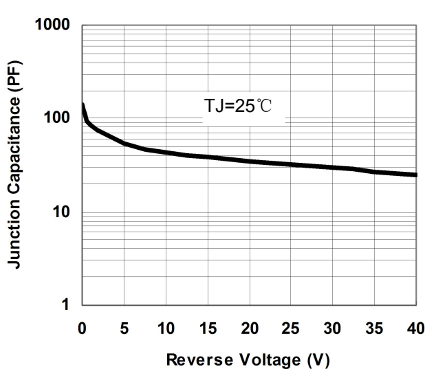
Fig.1-Typical Junction Capacitance
