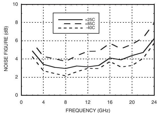
Noise Figure
