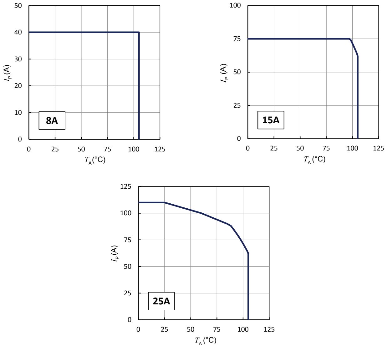
Figure 16: I_p vs T_A for HO series
