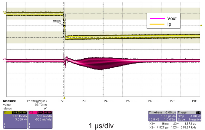
Figure 14: dv/dt
