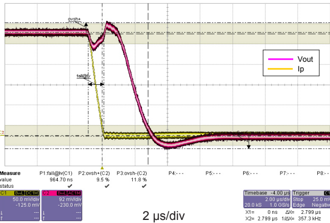
Figure 13: Step response
