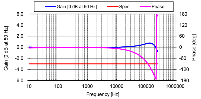
Figure 12: Frequency response
