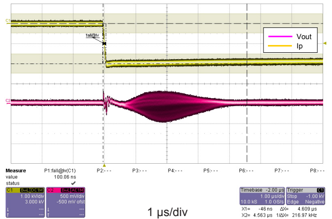
Figure 4: dv/dt
