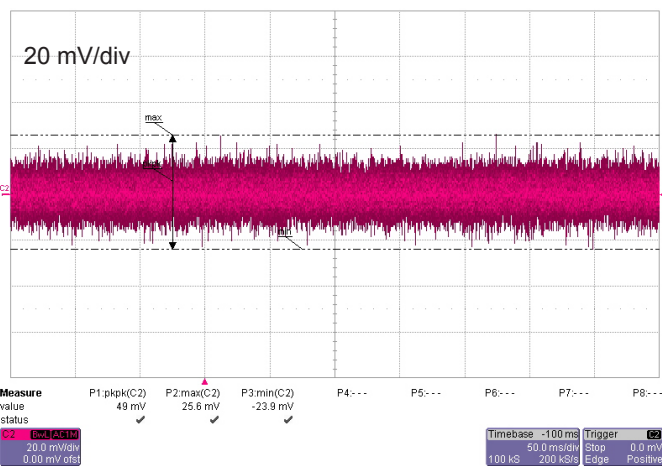
Figure 5: Output noise
