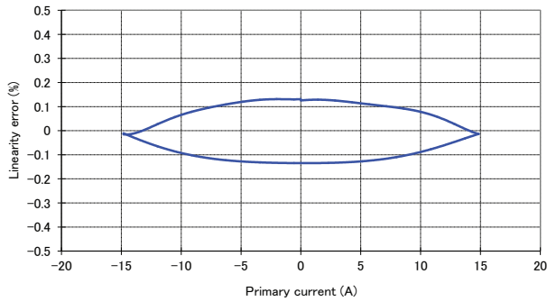
Figure 6: Linearity error
