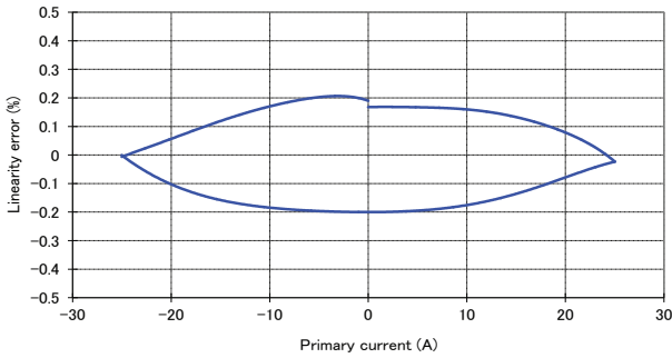
Figure 11: Linearity error
