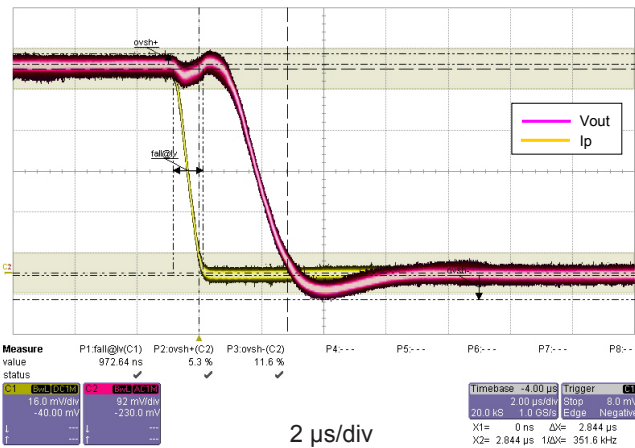
Figure 3: Step response
