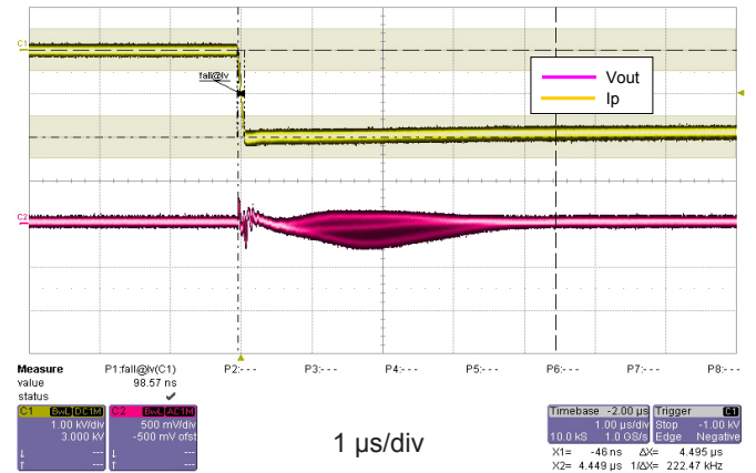
Figure 9: dv/dt
