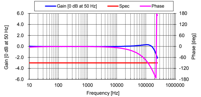
Figure 7: Frequency response
