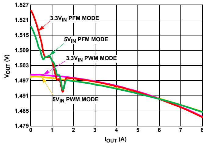
FIGURE 12. V_{OUT} REGULATION vs LOAD (1MHz, V_{OUT} = 1.5\text{V} )
