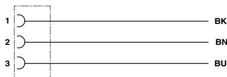
Contact assignment of 7/8" socket
