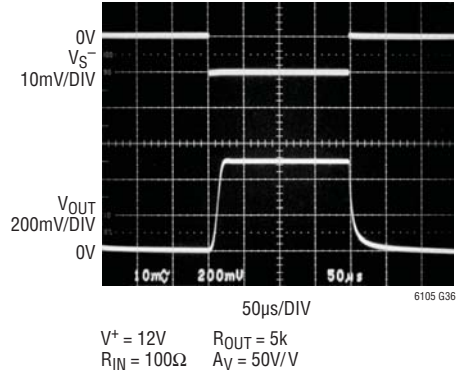
Step Response V_{SENSE} = 0V to 10mV , V_{S^+} = 0V
