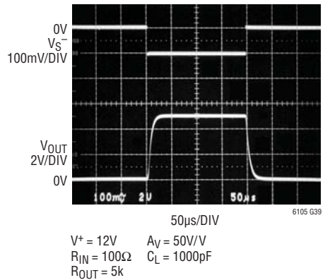
Step Response V_{SENSE} = 0V to 100mV , C_L = 1000pF , V_{S^+} = 0V
