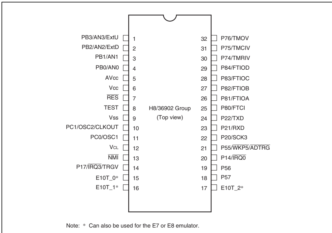
Figure 1.6 Pin Arrangement of H8/36902 Group (FP-32D, 32P4B)
