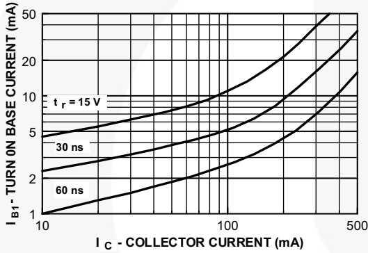
Figure 11. Rise Time vs. Collector and Turn-On Base Currents
