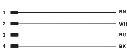
Contact assignment of the 7/8" plug
