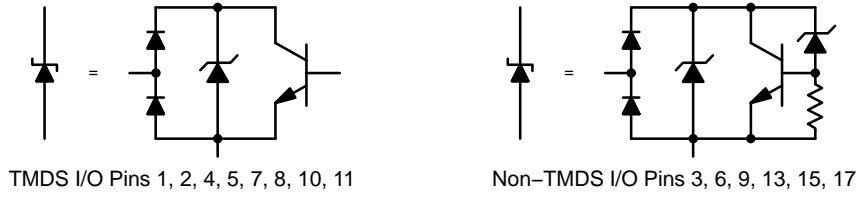
Figure 1. Pin Schematic
