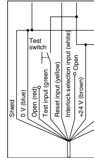
Wiring for use of the test function of the Light Curtain
