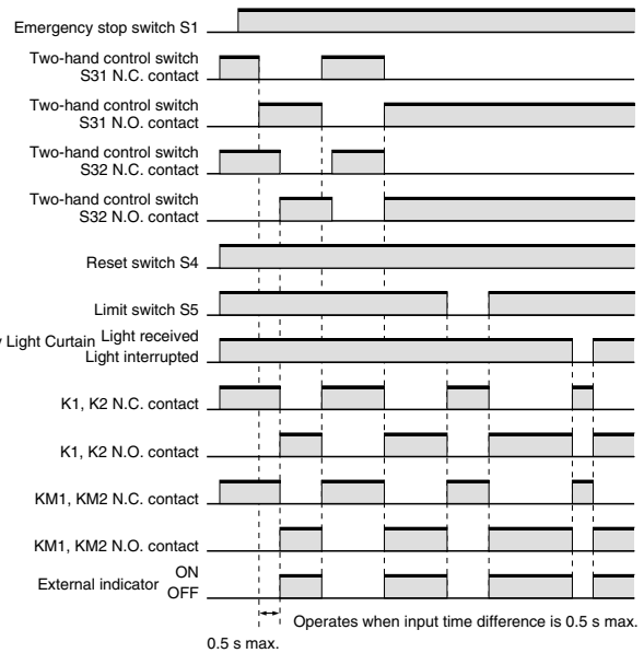
Timing Chart
