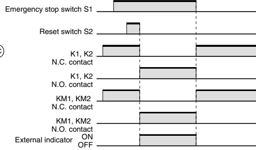
Timing Chart
