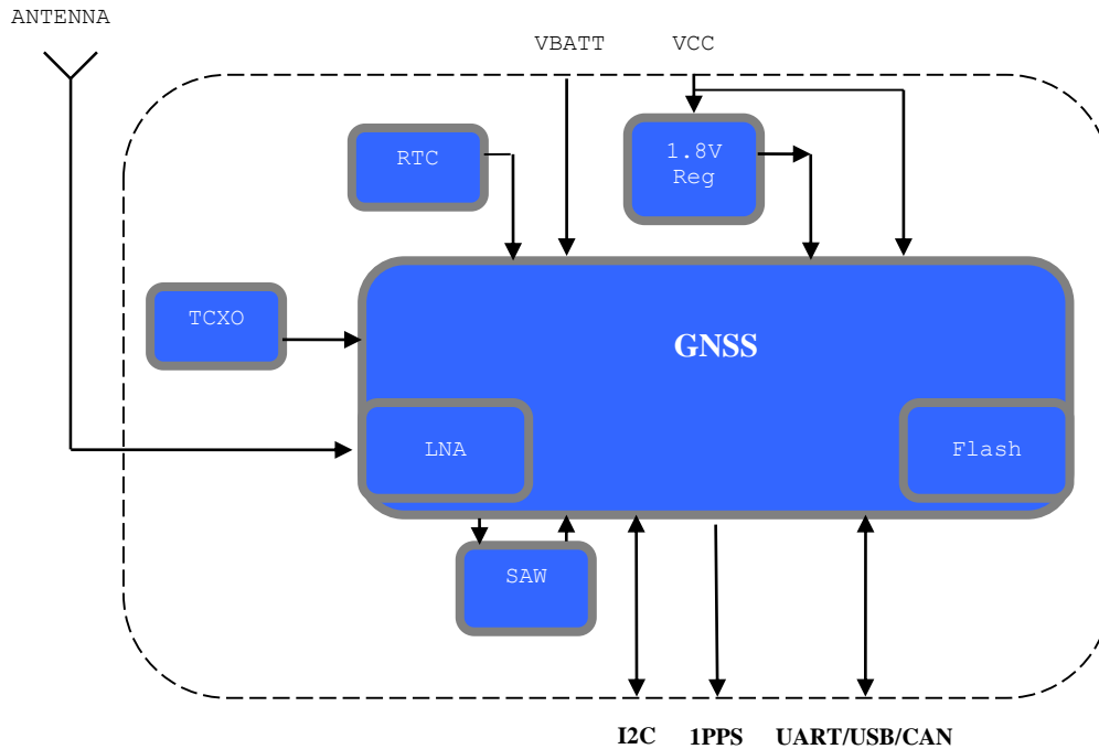
Figure 1 SL869 Architecture
