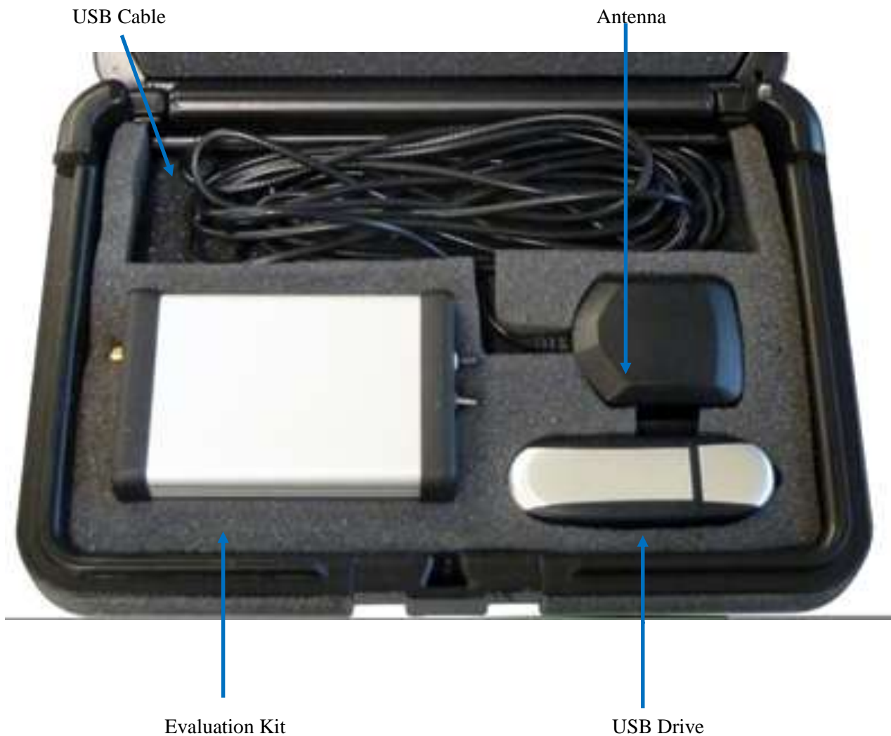
Figure 6 SL869 EVK
