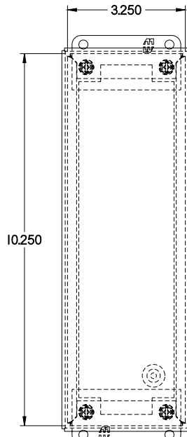
FRONT VIEW
