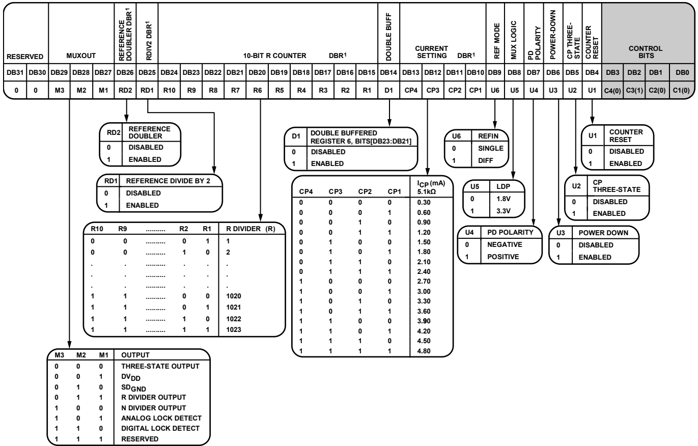
Figure 42. Register 4 Details
