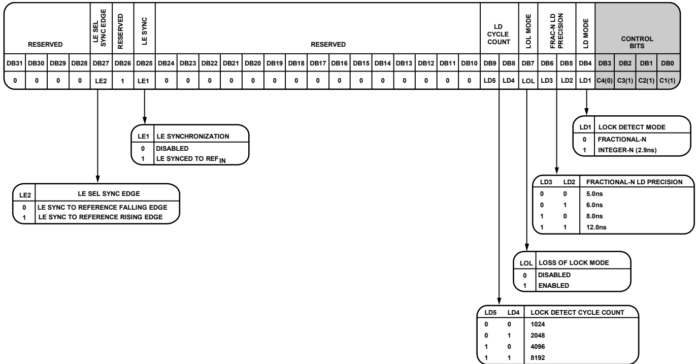
Figure 45. Register 7 Details
