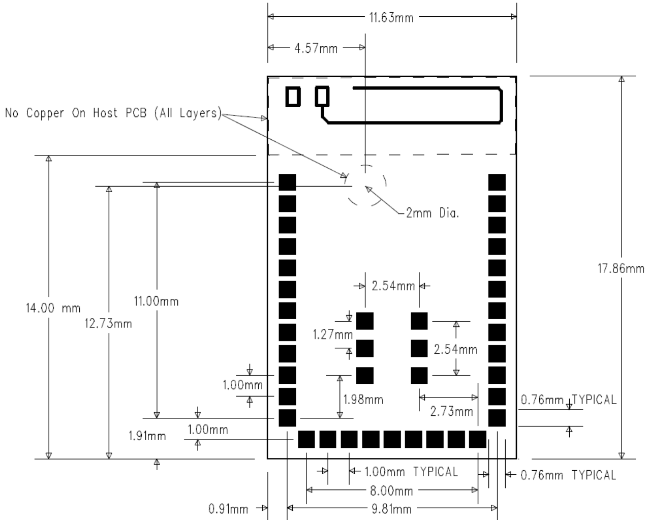
Figure 18: SaBLE-x-R2 Recommended PCB Footprint (Viewed from Top)
