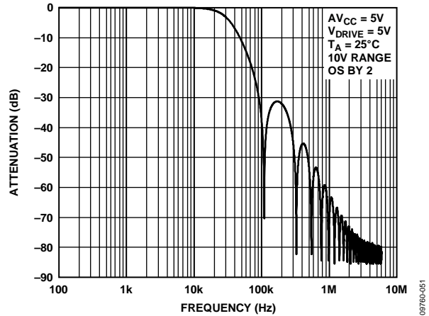
Figure 54. Digital Filter Response for OS x 2
