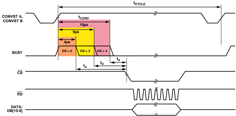
Figure 46. AD7609—No Oversampling, Oversampling × 4, and Oversampling × 8 Using Read After Conversion
