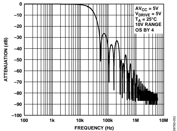
Figure 55. Digital Filter Response for OS x 4
