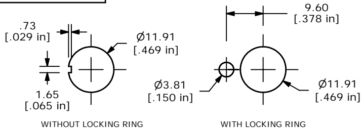
PANEL MOUNTING
