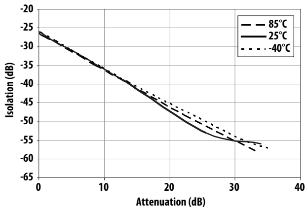
Figure 40. Isolation vs Attenuation and Temperature at 2500MHz
