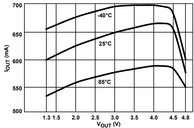
FIGURE 5. CURRENT REGULATION vs V OUT (V IN = 5V)
