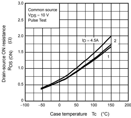
R_{DS(ON)} - T_c
