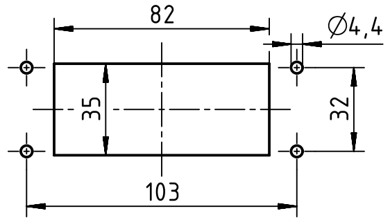
Panel cut out (1:2)
