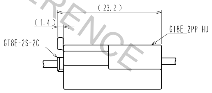
Mated Connectors
