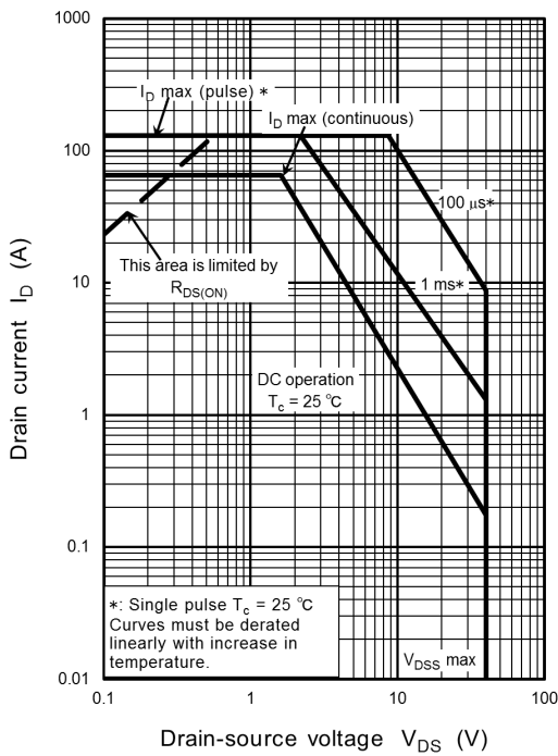
Fig. 8.13 Safe Operating Area (Guaranteed Maximum)
