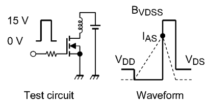
Fig. 8.15 Test Circuit/Waveform
