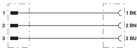
Contact assignment of 7/8" plugs/sockets
